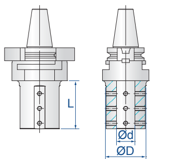
Boring Holder (BOB)
